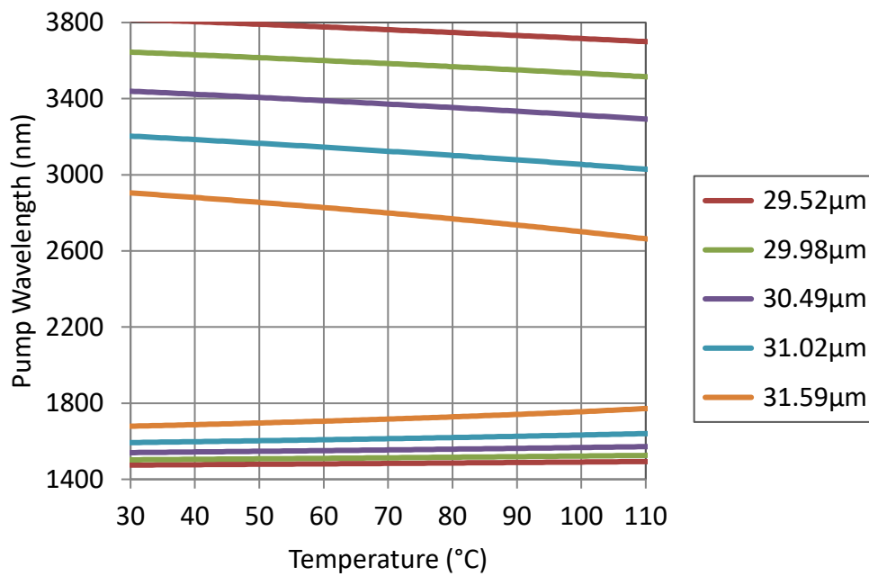
OPO Tuning Curve 1064nm Pump
