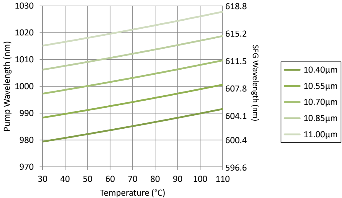
SFG Tuning Curve for 1550nm Pump
