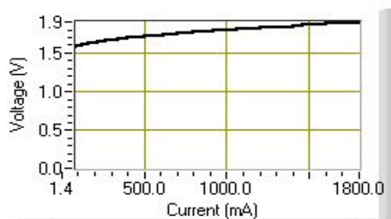
CW V-I curve
