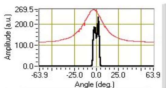
CW far field at 1800mA
