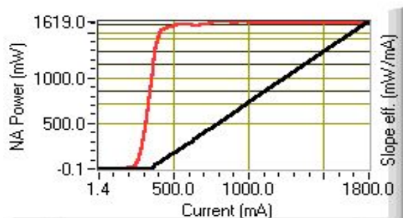
CW L-I, dL/dI curve
