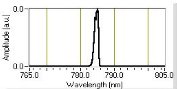
CW spectrum at 1500mW
