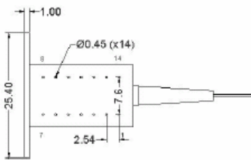
14-Pin DIL Package
