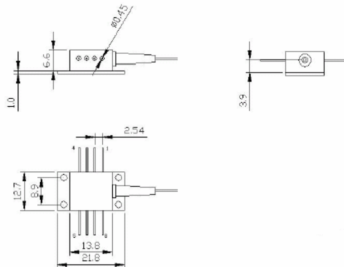
8-Pin BUT Package
