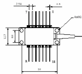
14-Pin BUT Package
