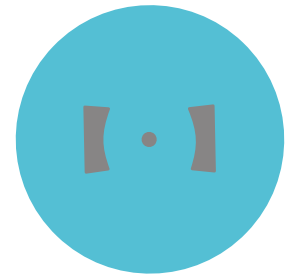
PM Coupler fiber end face diagram
